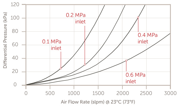
Linegard GIGAX-FP Filters
