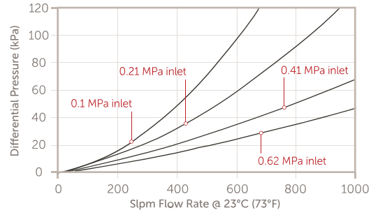
Wafergard MAX In-line (1/2" Fittings)
