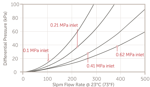
Wafergard MAX In-line (1/4" Fittings)
